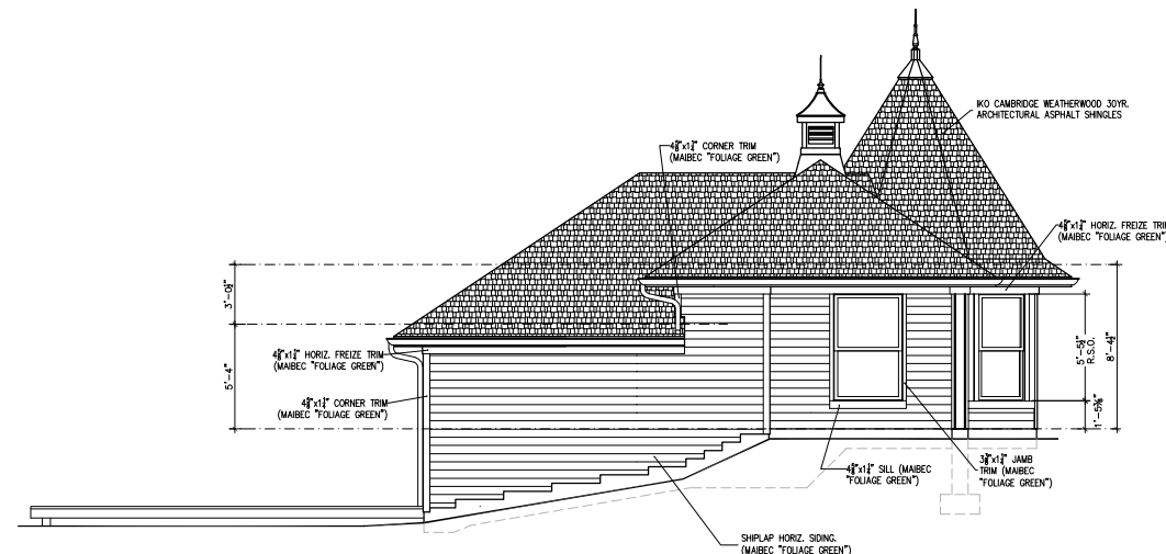
6 East Elevation A-1 Scale: 1/4"=1'
