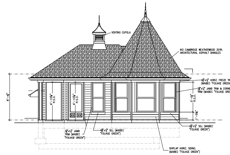
5 South Elevation A-1 Scale: 1/4"=1'
