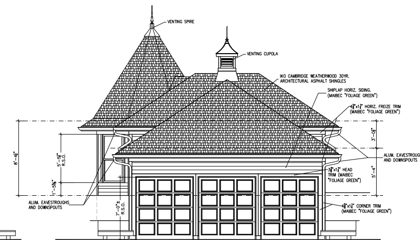
5 South Elevation A-1 Scale: 1/4"=1'
